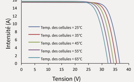
Intensité-Tension (460W)
