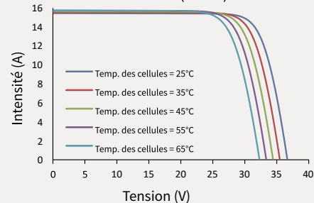
Intensité-Tension (460W)
